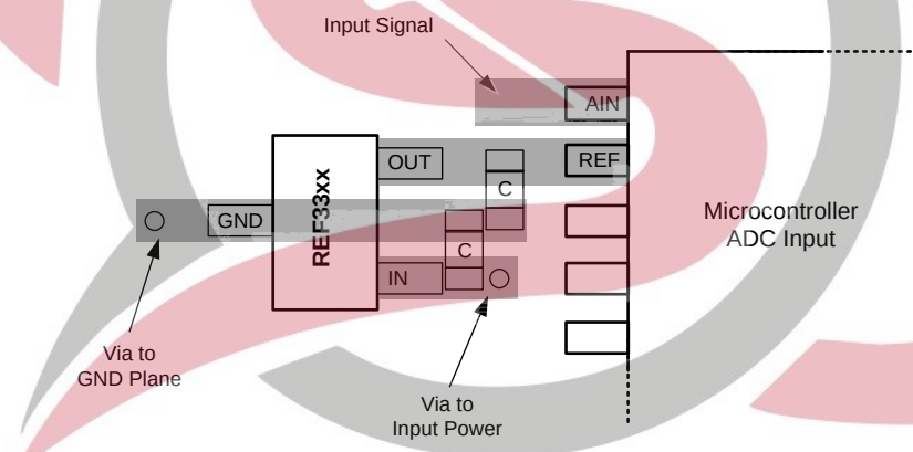
Figure 25. Layout Example
